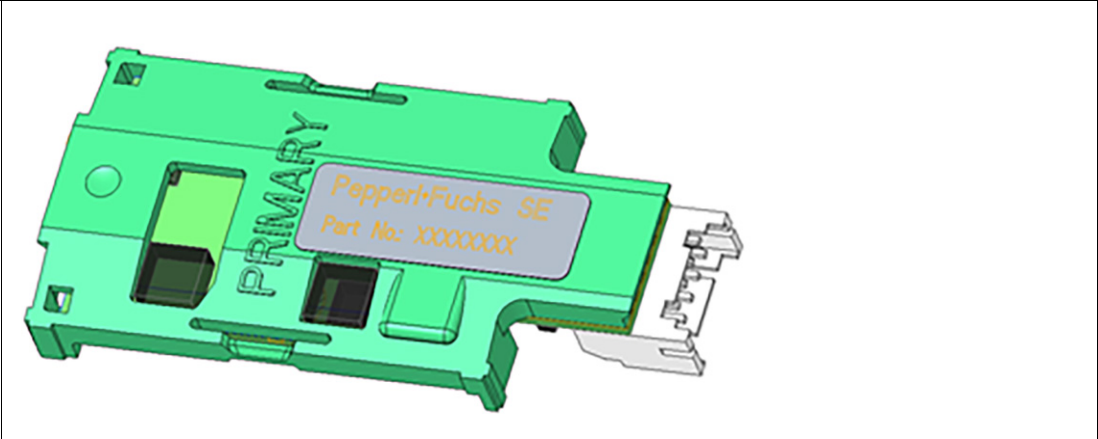
Figure 2.7 Both versions of the IO module can be fitted to a sensor module as desired. The sensor module with the IO module is the primary sensor. Either sensor module can become the primary sensor via an IO module. If both sensors are primary sensors, they must be taught in separately from each other without door hinge HS/HOS connecting cables.
