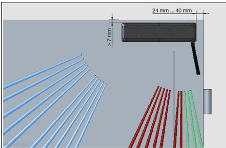
Figure 3.1 Position of device – door without door closer
