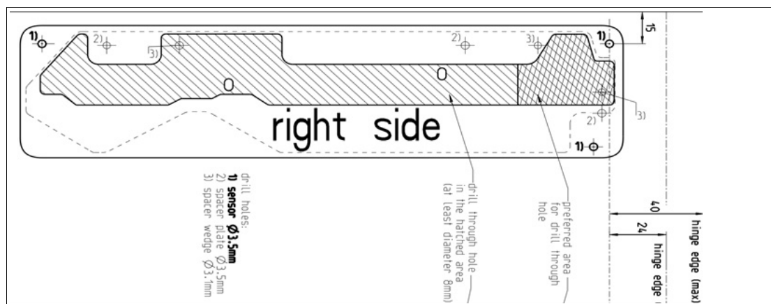
Figure 3.5 Drilling template
