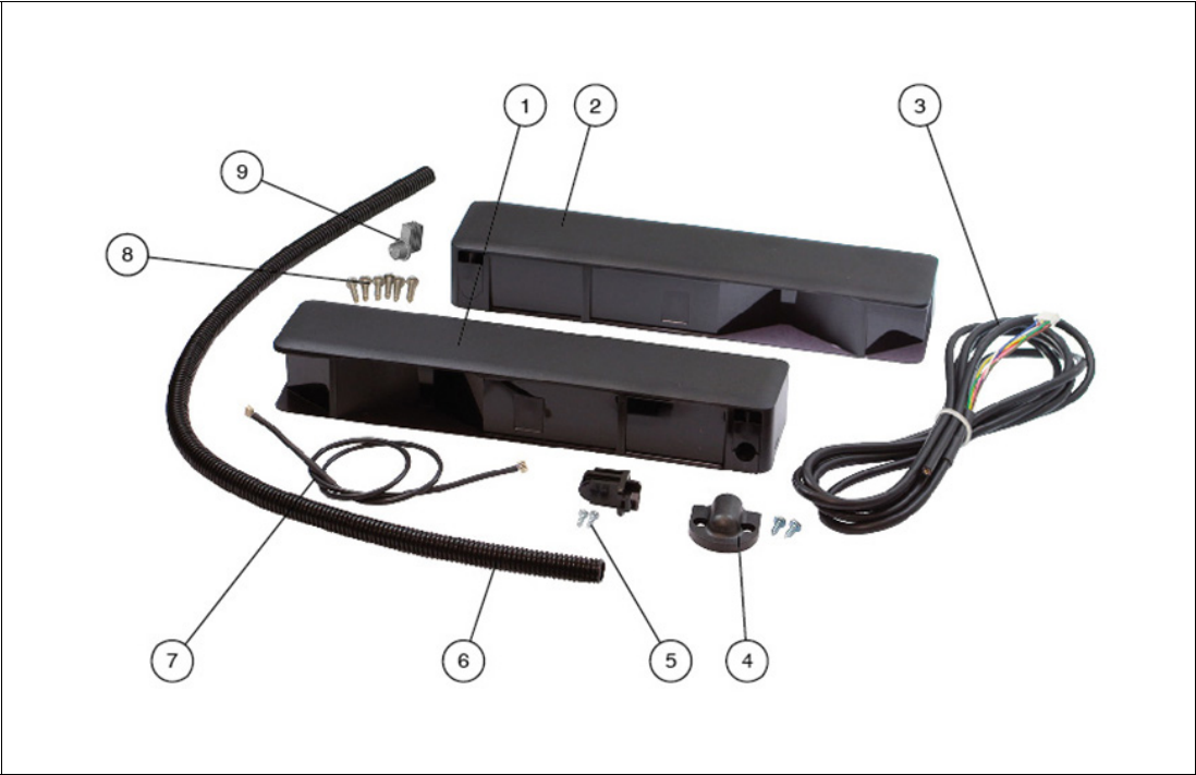
Figure 2.9 Scope of delivery
