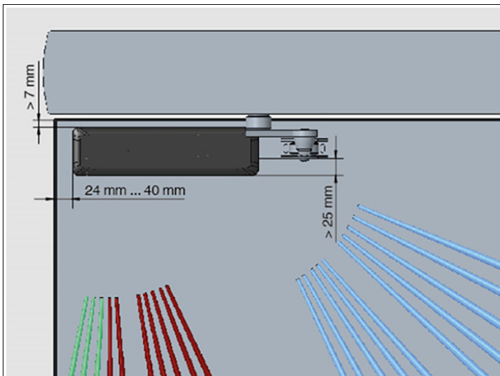
Figure 3.2 Position of device – door with scissor arm
