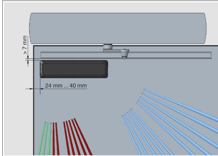
Figure 3.3 Position of device – door with slide rail
